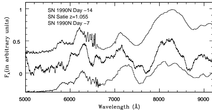
Figure 3: (a) 30'' \times 30'' section of our NIRI image centered on “Satie”, a supernova at z = 1.06 discovered in our search during semester 2001A. The combined (12 hr) NIRI image reaches S/N \sim 14 ; a final reference image with NIRI is needed to subtract host galaxy light. (b) Spectrum of “Satie” obtained in 2 hrs with ESI on Keck, smoothed to 155 \text{ \AA} , and compared to the nearby template SN1990N.
