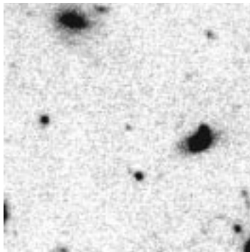
Figure 3: (a) 30'' \times 30'' section of our NIRI image centered on “Satie”, a supernova at z = 1.06 discovered in our search during semester 2001A. The combined (12 hr) NIRI image reaches S/N \sim 14 ; a final reference image with NIRI is needed to subtract host galaxy light. (b) Spectrum of “Satie” obtained in 2 hrs with ESI on Keck, smoothed to 155 \text{ \AA} , and compared to the nearby template SN1990N.
