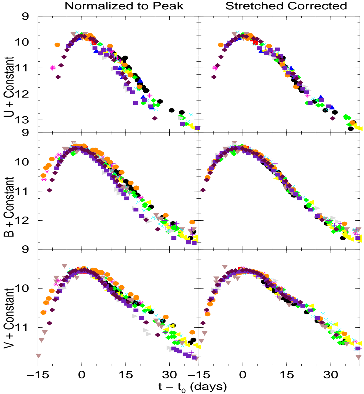
Fig. 2.— Left panels: The UBV -band light curves of several nearby SNe Ia adjusted to the same peak magnitude. Right panels: The same light curves corrected by their B -band stretch factor. Note the large reduction in scatter about the mean.
