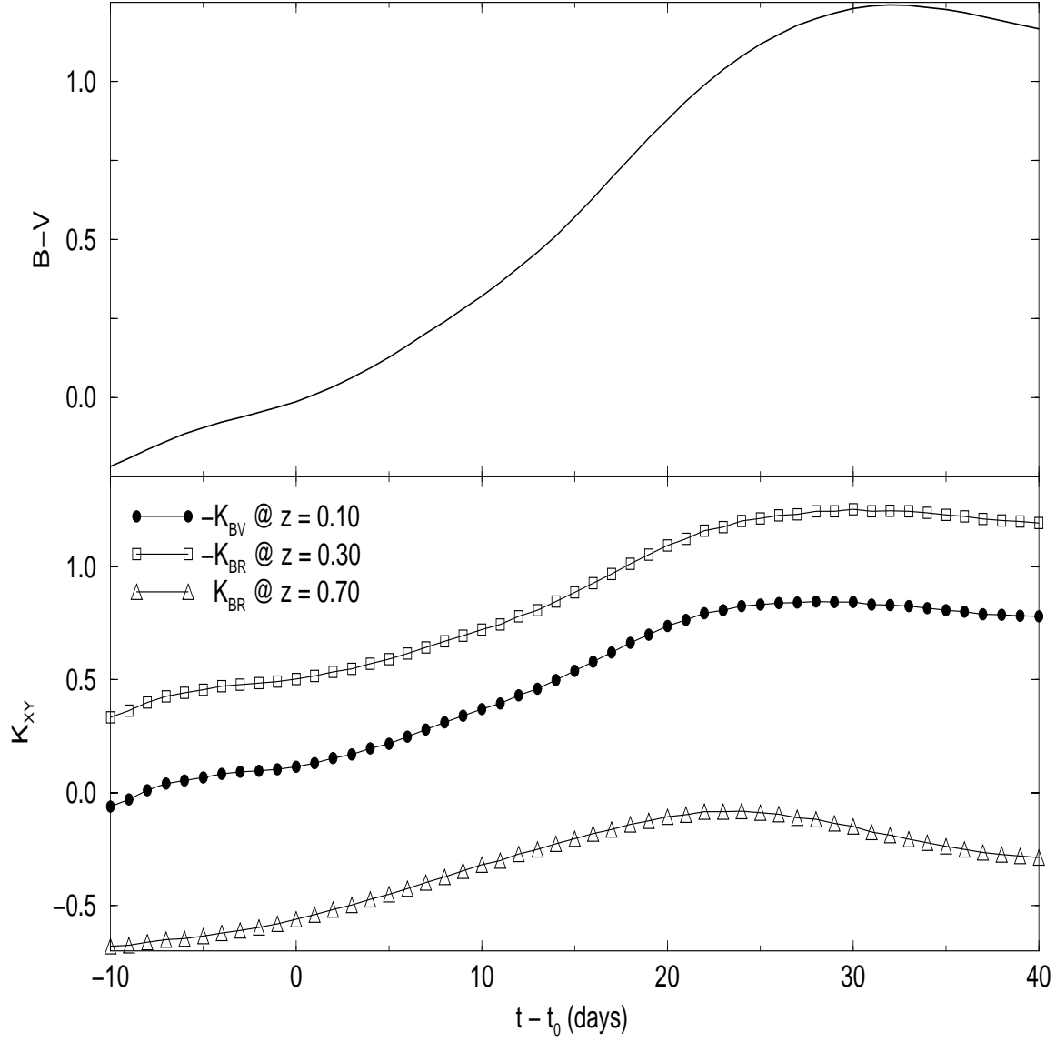
Fig. 3.— Top panel: Rest-frame B-V color curve for a s = 1.0 SN Ia. Bottom panel: K -corrections for a s = 1.0 SN Ia at a variety of redshifts. Note the strong similarity between the color curve and the K -corrections.
