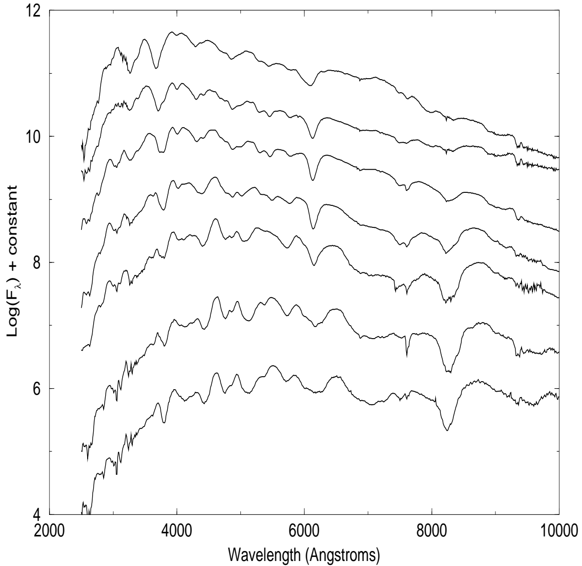
Fig. 6.— A weekly sampling of the spectral template from two weeks before to four weeks after maximum light. The spectra and light curves are available at: http://www.supernova.lbl.gov/~nugent/spectra.html
