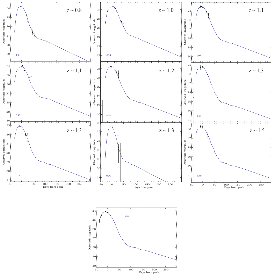
Figure 2. Upper Array of Plots: The i' -band lightcurves for the nine supernovae targeted by this proposal (red points in the Figure 1 lower inset). Each of these SNe also has R- and z' -band photometry points near maximum light (not shown). Note that for these nine SNe the integrated host galaxy light in a 1'' aperture is significantly brighter than the SN in almost every case. Lower Panel: The i' -band lightcurve for the unusual target “058.” The peak magnitude of this target is over a magnitude brighter than expected for a SN Ia at the redshift ( z > 1.5 ) indicated by its lightcurve time dilation.
