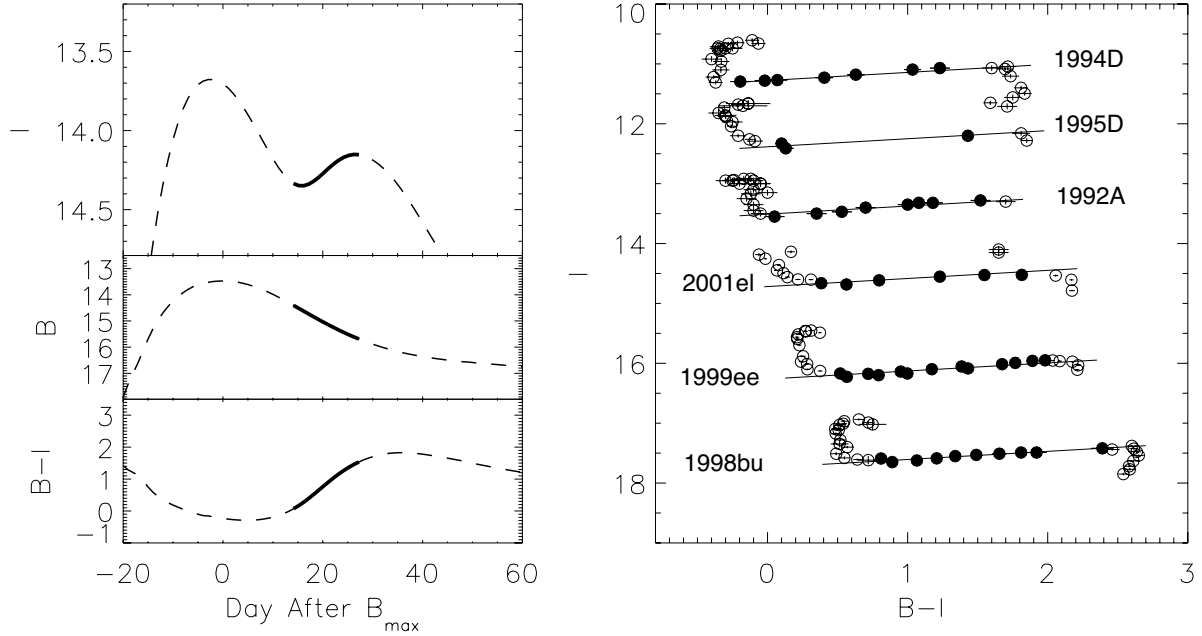
Figure 2: Illustrations of the CMAGIC method. Left panel, from top to bottom, the I-Band and B-band light curves, and the B-I color curve for a normal supernova are shown. The solid line on the left panel shows the regions where B vs B-I can be described by a linear relation. The B vs B-I Color-Magnitude Diagram for several example SNe Ia are shown on the right panel, ordered by host-galaxy extinction going from top to bottom. Only data taken between 0 to 35 days after B_{max} are shown here. The data shown as solid dots correspond to epochs during which the relation between magnitude and color is linear for all SNe (this is 14–29 days after B_{max} for B-I for a typical supernova, and scales inversely with \delta m_{15} ). The linear region shows that the B and I band magnitudes are highly correlated. Observations of a single point in I band within the window where the linear relation holds true would be sufficient to describe accurately the I -band light curves in the linear region. Using this linear relation we define fiducial magnitudes, which are found to be better distance indicators than maximum-light magnitudes (Wan03). It was shown that that the slopes of the linear relation are identical for all well-observed nearby SNe, thus a single slope can be used for all SNeIa.
