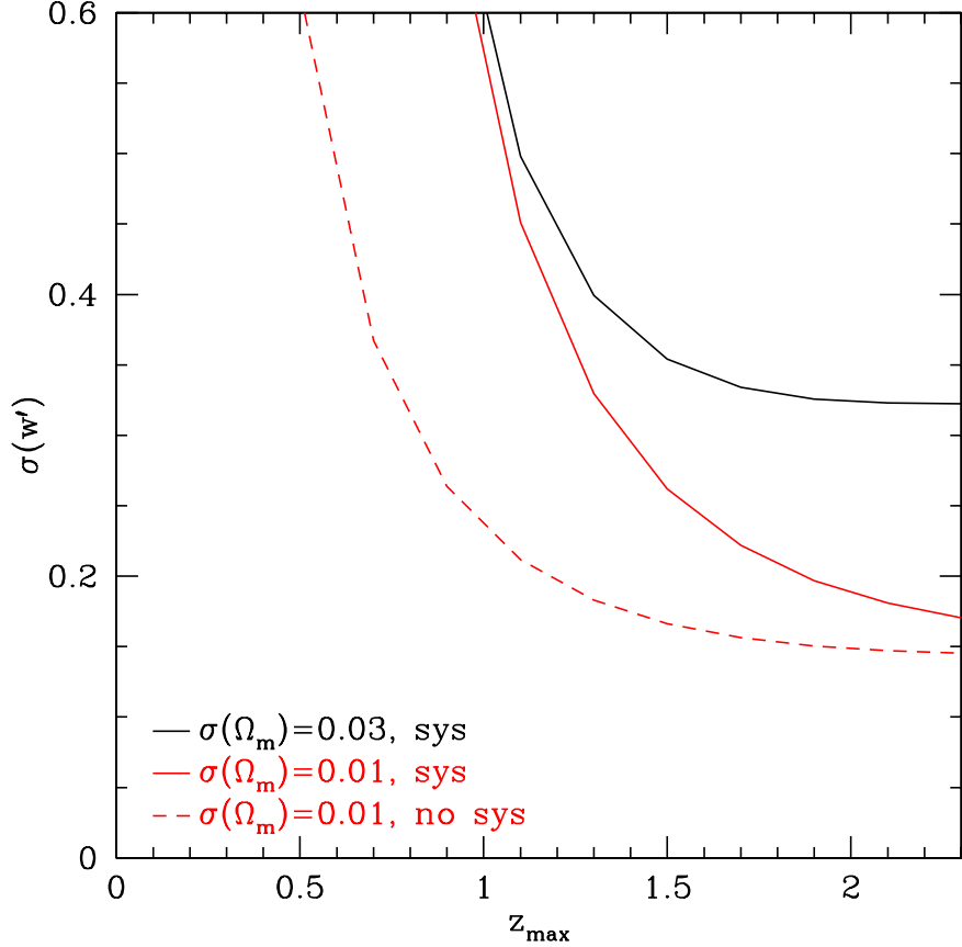
Figure 1: Comparisons of simulated measurements of the time variation of w , the dark-energy equation of state ratio. The measurements are based on a simulated Hubble diagram for SNe Ia that extends out to redshift z_{\max} . The uncertainty in this measurement, \sigma(w') improves significantly as the redshift range of the SN sample increases, until it levels off around z = 1.7 for a realistic scenario with systematic uncertainties (at a level achievable with future instruments currently being designed), and a prior on \Omega_M with 0.03 uncertainty. Less realistic scenarios with even better prior knowledge of \Omega_M (and possibly an idealized supernova and idealized measurements, i.e. no systematic uncertainties) give uncertainties in w' that level off around z = 1.5 or 2.3.
