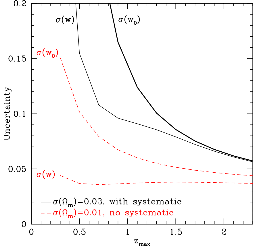
Figure 1: The dependence on the measurement uncertainty of the dark energy equation of state, w , as a function of the maximum redshift of a SN dataset — assuming a uniformly populated Hubble diagram to that redshift but a fixed total number of SNe. Cases are shown for a constant w and a time-varying w , for different levels of systematic error and assumed knowledge of \Omega_M from other experiments. Systematic errors will push SN Ia cosmological measurements to high redshift.
