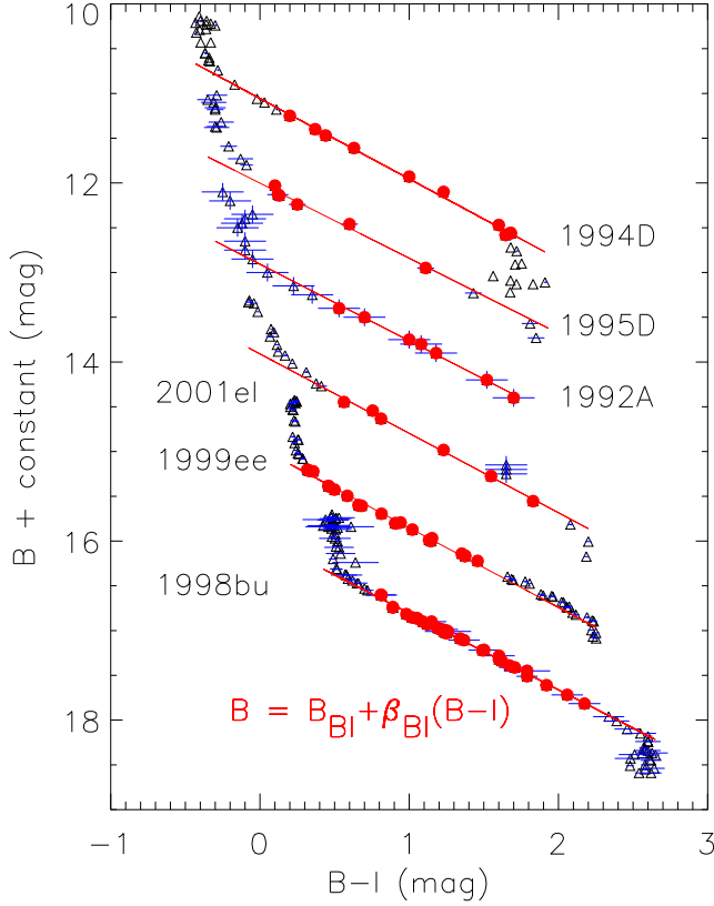
Figure 2: The B vs B-I Color-Magnitude Diagram for several example SNe Ia ordered by host-galaxy extinction going from top to bottom. The triangles show data points taken 0 to 35 days after B_{max} . The data shown as large red dots correspond to epochs during which the relation between magnitude and color is linear of all SNe (this is 13–25 days after B_{max} for B-I ). Using this linear relation we define fiducial magnitudes, which are found to be better distance indicators than maximum-light magnitudes (Wan03). Note that a single slope can be used for all SNeIa.
