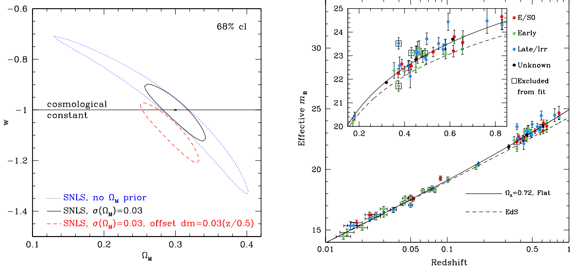
Figure 1: Figure 1a (Left): Projected 68% statistical confidence intervals on the dark energy equation of state possible from SNLS when it is completed 5 years from now, assuming a flat universe (from CMB measurements), and with (black-solid) and without (blue-dot) a prior of \Omega_M from Large-Scale Structure. If a small systematic error is introduced, the statistical confidence interval will miss the correct simulated \Lambda ( w = -1 ) solution by 2\sigma (red-dash). Figure 1b (Right): Our major new result based on several Cycles of HST data showing the stretch-corrected SNe Ia Hubble diagram for the SCP dataset plotted according to the class of the host galaxy. The inset shows the high-redshift SNe, the main panel the Hubble diagram for the entire sample. SNe Ia in E/S0 host galaxies show significantly less scatter than those in later types, and the E/S0 and spirals give values of \Omega_\Lambda and \Omega_M for a flat universe which agree to within their 0.1 uncertainty (Sul03).
