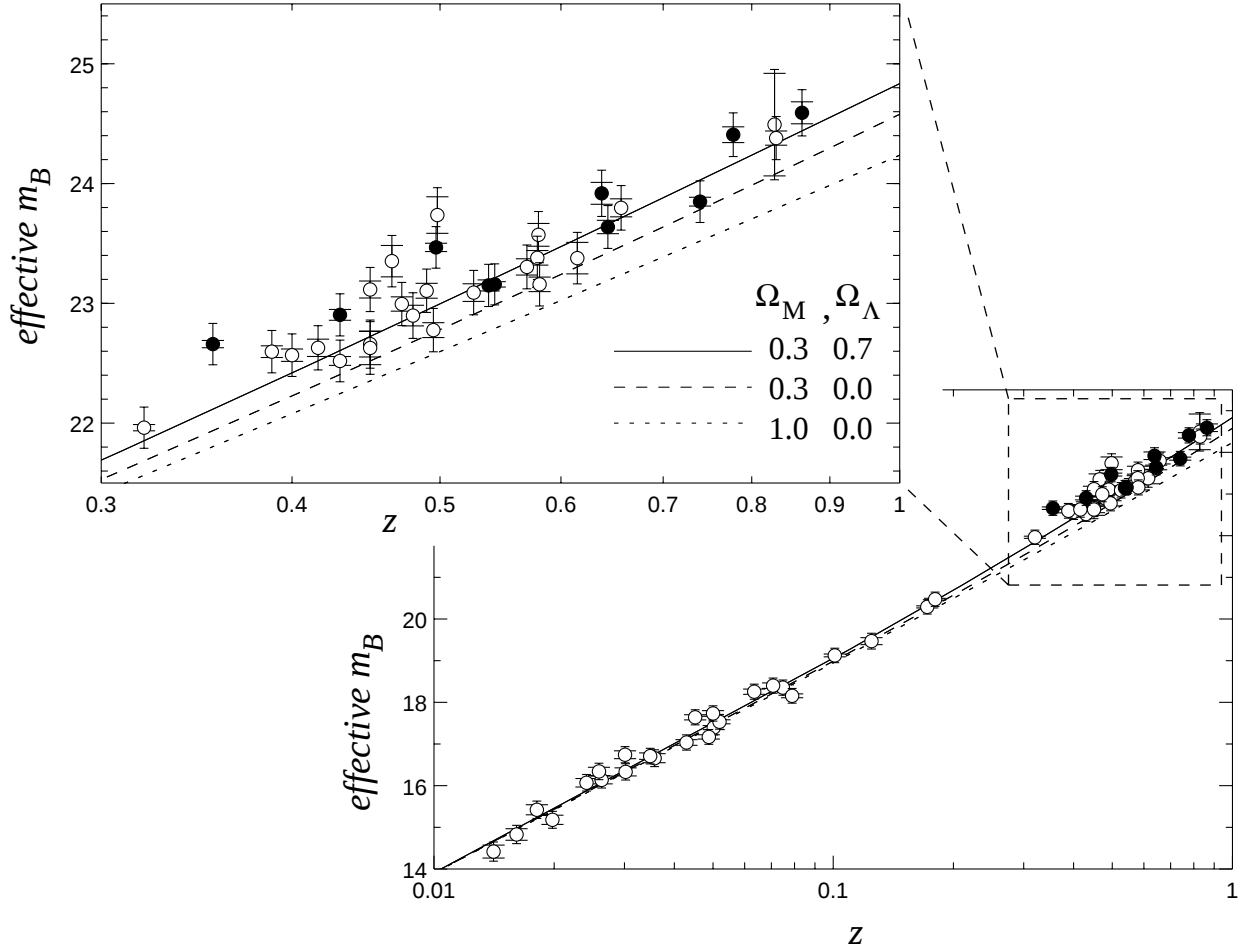
Fig. 5.— Hubble diagram of effective K - and stretch-corrected m_B vs. redshift for the supernovae in the full primary subset. Filled circles represent the HST supernovae of this paper. Note that two of the HST SNe are mildly reddened; see Figure 6. Inner error bars show just the measurement uncertainties; outer error bars include 0.17 magnitudes of intrinsic dispersion.
