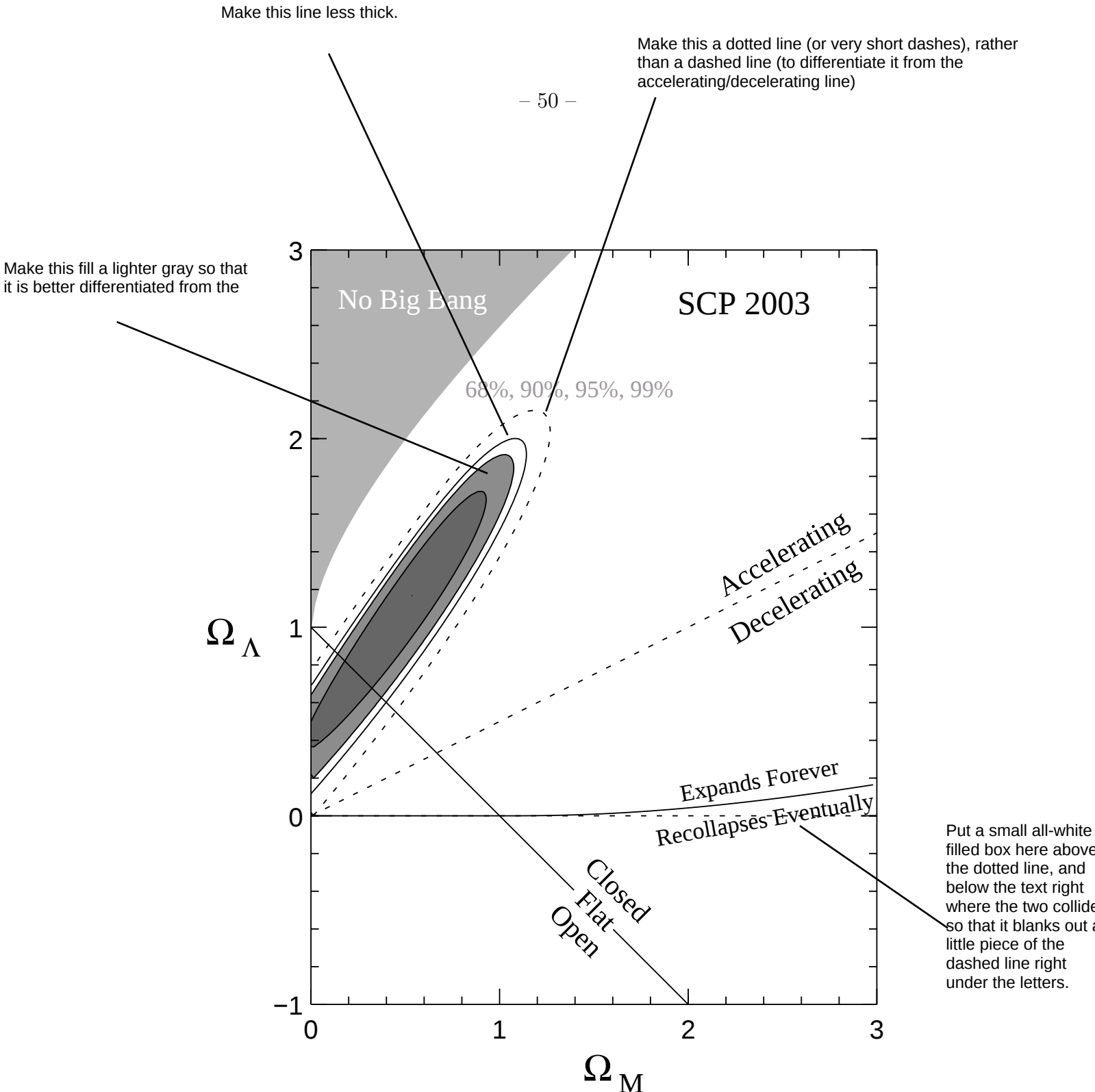
Fig. 7.— Primary 68%, 90%, 95%, and 99% confidence regions for \Omega_M and \Omega_\Lambda from a fit to the low-extinction primary subset (Fit 3).
