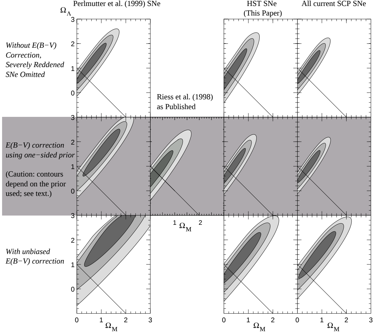
Fig. 9.— 68.3%, 95.4%, and 99.7% confidence regions for \Omega_M and \Omega_\Lambda using different data subsets and methods for treating host-galaxy extinction corrections. The top row represents our fits to the low-extinction primary subset, where significantly reddened supernovae have been omitted and host-galaxy extinction corrections are not applied. The second row shows fits where extinction corrections have been applied using a one-sided extinction prior. These fits are sensitive to the choice of prior, and can either yield results equivalent to analyses assuming low extinction (but without testing the assumption), or yield biased results (see text). Note that the published contours from Riess et al. (1998, their Fig. 6, solid contours) presented results from fits that included not only well-observed supernovae, but also four supernovae with very sparsely sampled lightcurves, one supernova at z = 0.97 without a spectral confirmation, as well as two supernovae from the P99 set. The third row shows fits with unbiased extinction corrections applied to our primary subset. The HST SNe presented in this paper show a marked improvement in the precision of the color measurements, and hence in the precision of the \Omega_M and \Omega_\Lambda measurements when a full extinction correction is applied. With full and unbiased extinction corrections, dark energy is still required with P(\Omega_\Lambda > 0) = 0.99 .
