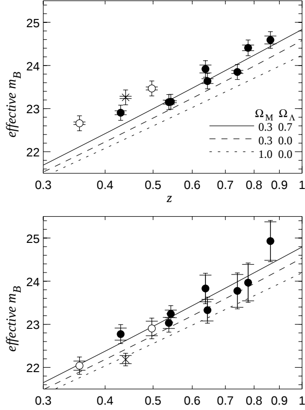
Fig. 6.— Hubble diagram of effective K - and stretch-corrected m_B vs. redshift for the 11 supernovae observed with WFPC2 and reported in this paper. Circles represent supernovae in the primary subset (Subset 1); the one point plotted as a cross (the very reddened supernova SN 1998aw) is omitted from that subset. Open circles represent reddened supernovae omitted from the low-extinction primary subset (Subset 2), while filled circles are in both Subsets 1 and 2. Upper plot: no host-galaxy E(B-V) extinction corrections have been applied. Inner error bars only include the measurement error. Outer error bars include 0.17 magnitudes of intrinsic dispersion. Lower plot: extinction corrections have been applied using the standard interstellar extinction law. Error bars have been increased by the uncertainty in this extinction correction. Again, inner error bars represent only measurement uncertainties, while outer error bars include 0.11 magnitudes of intrinsic dispersion. Lines are for three example cosmologies with the indicated values of \Omega_M and \Omega_\Lambda .
