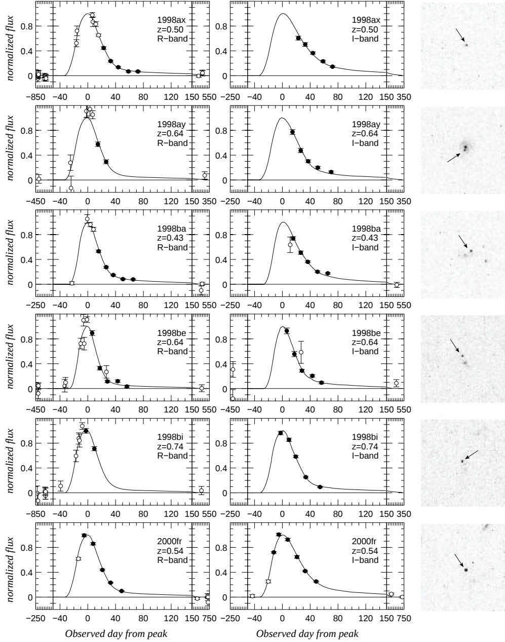
Fig. 2.— Lightcurves and images from the PC CCD on WFPC2 for the HST supernovae reported in this paper (continued). The left column shows the R -band (including F675W HST data), the middle column I -band lightcurves (including F814W HST data), and the right column 7'' × 7'' F675W images of the supernovae. Open circles represent ground-based data points, and filled circles represent WFPC2 data points.
