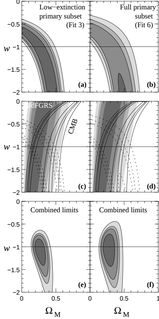
Fig. 11.— Joint measurements of \Omega_M and w assuming \Omega_M + \Omega_X = 1 and that w is not time-varying. Confidence regions plotted are 68%, 90%, 95%, and 99%. The left column (panels a, c, and e) shows fits to the low-extinction primary subset; the right column (panels b, d, and f) shows fits to the primary subset with unbiased individual host-galaxy extinction corrections applied to each supernova. The upper panels (a and b) show the confidence intervals from the SCP supernovae alone. The middle panels (c and d) overlay this (dotted lines) with measurements from 2dFGRS (filled contours) (Hawkins et al. 2002) and combined CMB measurements (solid contours) (Bennett et al. 2003; Spergel et al. 2003). The bottom panels (e and f) combine the three confidence regions to provide a combined measurement of \Omega_M and w .
