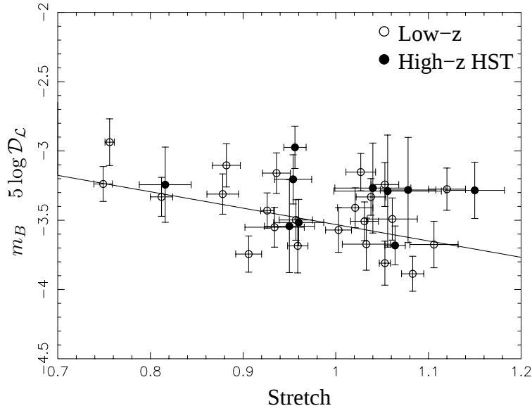
Fig. 13.— Stretch-luminosity relationship for low-redshift SNe (open circles) and high-redshift HST SNe (filled circles). Each point is the K -corrected m_B for that supernova, minus \mathcal{D}_L , the “Hubble-constant-free luminosity distance” (see § 2.4), plotted against the stretch of that SN. The line drawn represents the best-fit values of \alpha and \mathcal{M} from Fit 6, the fit to all Subset 1 supernovae with host-galaxy extinction corrections applied. Note in particular that our HST SNe Ia all have low-redshift counterparts.
