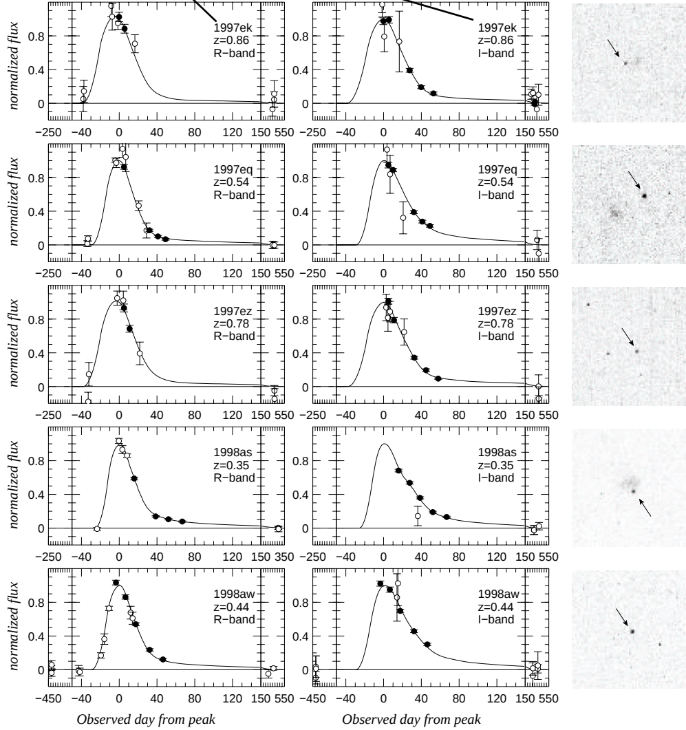
Fig. 1.— Lightcurves and images from the PC CCD on WFPC2 for the HST supernovae reported in this paper. The left column shows the R -band (including F675W HST data), the middle column I -band lightcurves (including F814W HST data), and the right column 7'' \times 7'' F675W images of the supernovae. Open circles represent ground-based data points, and filled circles represent WFPC2 data points.
