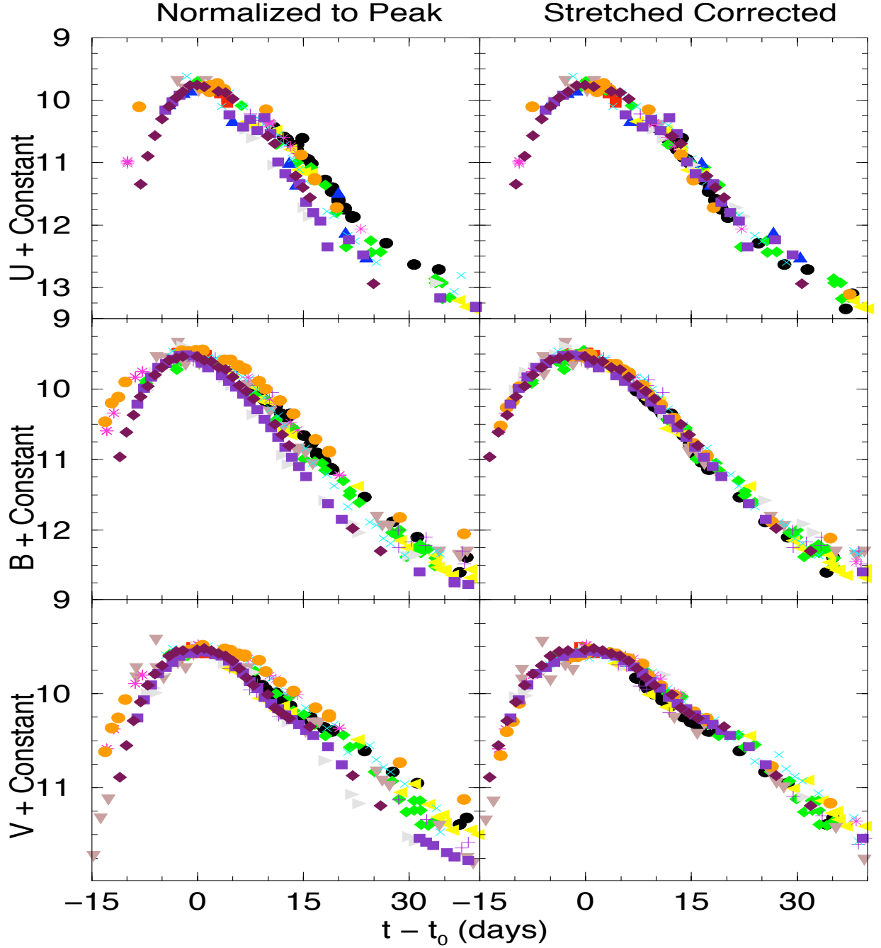
Fig. 2.— Left panels: The UBV -band light curves of several nearby SNe Ia adjusted to the same peak magnitude. Right panels: The same light curves corrected by their B -band stretch factor. Note the large reduction in scatter about the mean.
