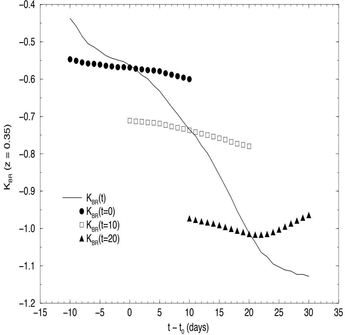
Fig. 5.— K_{BR} for a z = 0.35 SN Ia with s = 1.0 along with three other sets of K -corrections. These K -corrections were calculated by forcing the spectra within 10 days of a given epoch on the light curve (maximum light, +10 days and +20 days) to have the same colors as the SN Ia has at that epoch. The difference in the K -corrections is, at most, 0.05 mag over the entire 20 day window and \lesssim 0.02 mag for a 10 day window.
