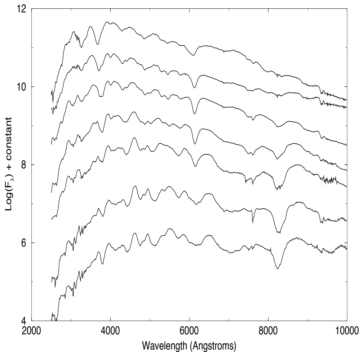
Fig. 6.— A weekly sampling of the spectral template from two weeks before to four weeks after maximum light. The spectra and light curves are available at: http://www.supernova.lbl.gov/~nugent/spectra.html
