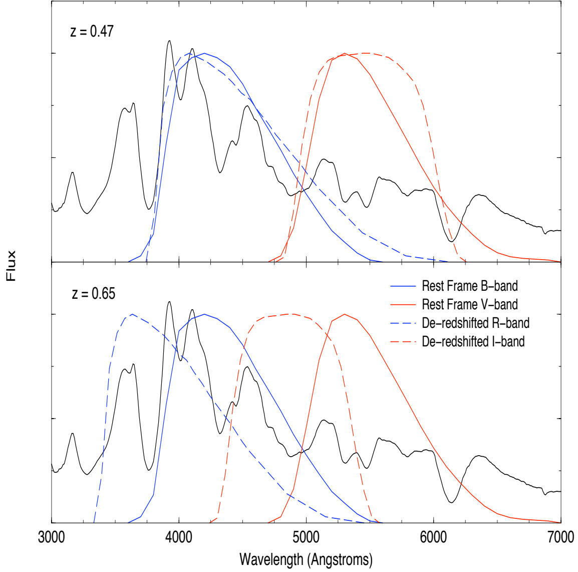
Fig. 1.— Filter pairings for R - and I -band observations of a redshifted SN Ia near maximum-light with respect to rest-frame B - and V -band filters. Nice matches occur at z = 0.47 while large extrapolations occur at z = 0.65 .
