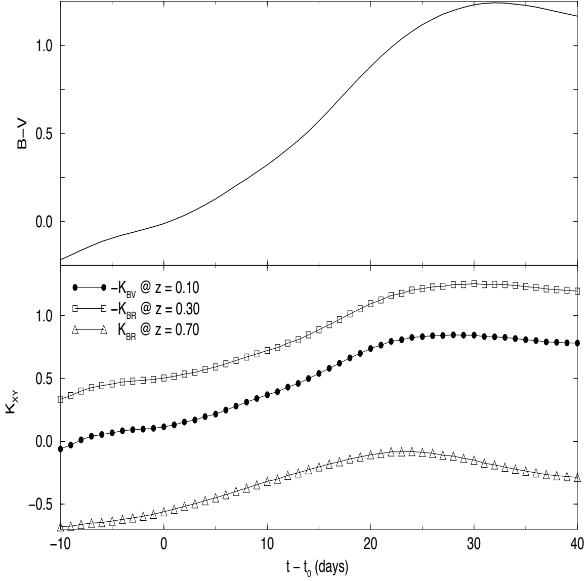
Fig. 3.— Top panel: Rest-frame B - V color curve for a s = 1.0 SN Ia. Bottom panel: K -corrections for a s = 1.0 SN Ia at a variety of redshifts. Note the strong similarity between the color curve and the K -corrections.
