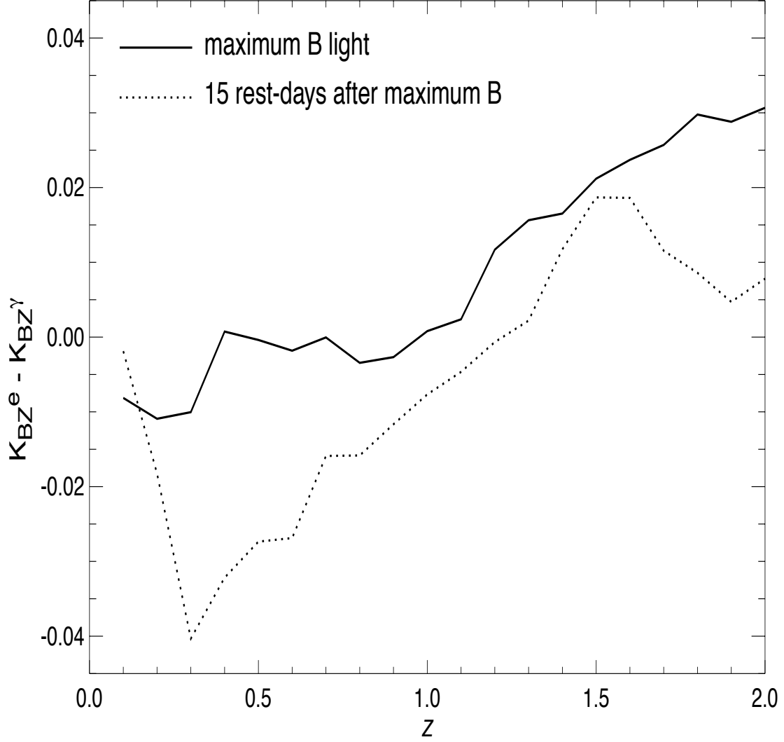
Fig. 15.— K_{BZ}^e - K_{BZ}^\gamma for a standard Type Ia supernova at B maximum and 15 days after maximum as a function of redshift. Measurements in I and bluer filters for z < 1 supernovae and J and redder filters for z > 1.5 would provide a better match of observed spectral regions.
