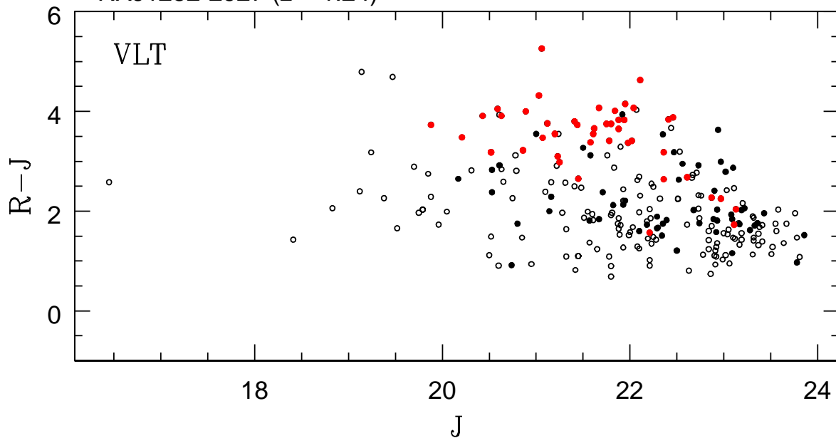
RXJ1252-2927 ( z = 1.24 )
