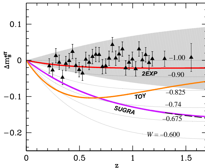
FIG. 5: Simulated binned data, with solid curves from a Supergravity inspired model [3, 4] (with the best w_0 - w_1 expansion fit shown as a dashed line, mostly covered by the solid SUGRA line), a strongly evolving toy model with w_0 = -0.6 and w_1 = -0.8 ( TOY ), and a model involving two exponentials [10] ( 2EXP ). A range of constant w models is shown as a grid of dotted lines. The shaded region corresponds to cosmological constant models with 0.25 \leq \Omega_m \leq 0.35 . The plot is taken from [6].
