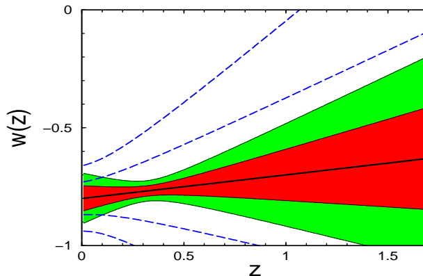
FIG. 2: 68% and 95% c.l. constraints on w(z) using simulated SNAP data, assuming a linear expansion of w in redshift and around a fiducial model w(z) = -0.8 + 0.1z . The shaded regions assume a perfectly known \Omega_M , while the dashed lines show the effect of assuming a Gaussian uncertainty of 0.05 in \Omega_M . The plot is taken from Ref. [8].
