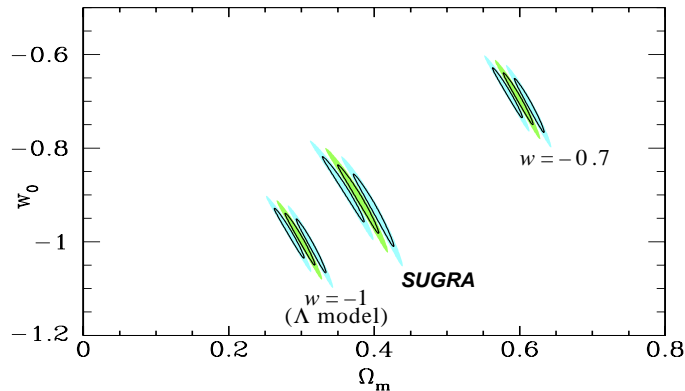
FIG. 6: Separation of dark energy models (labeled as in Fig. 5) in the \Omega_m - w_0 plane. We show 39.3% ( \Delta\chi^2 = 1 , shown as solid-line contours) and 68% ( \Delta\chi^2 = 2.3 , shown as shaded contours) confidence regions which project on the axes to give marginalized 1\sigma and 1.5\sigma errors respectively. The left and right flanking contours for each model show the effects of a drifting systematic error (see text). The w = -0.7 model has \Omega_m = 0.6 . This plot is from [6].
