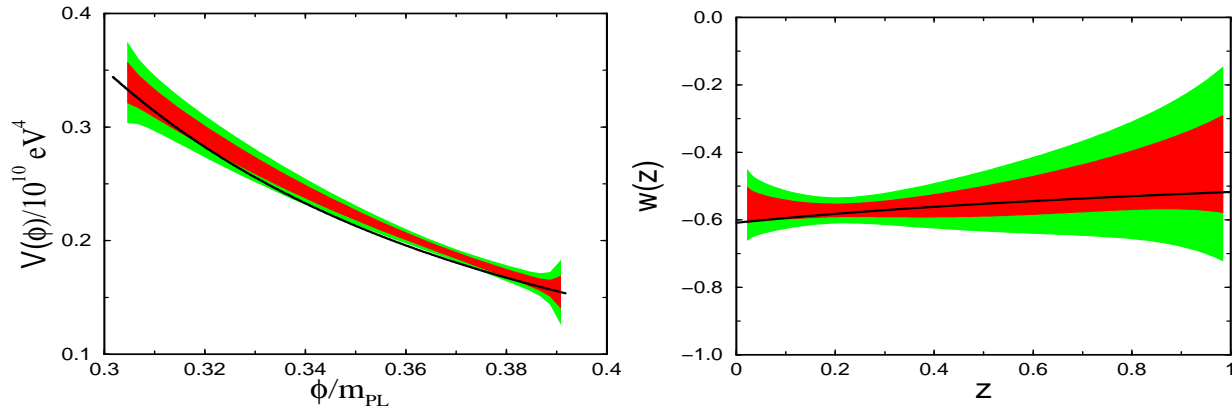
FIG. 8: Reconstruction of the quintessence model with potential V(\phi) = M^4[\exp(m_{\text{PL}}/\phi) - 1] [3] and \Omega_\phi = 0.50 . The solid line is the input model, and the shaded regions show the 68% and 95% confidence, produced from Monte Carlo simulation of 2000 SNe uniformly distributed out to z = 1.5 with individual uncertainties of 0.15 mag (7% in distance). A three-parameter Padé approximant fit to r(z) was used. The right panel shows the reconstruction of w(z) = (\frac{1}{2}\dot{\phi}^2 - V)/(\frac{1}{2}\dot{\phi}^2 + V) . The plot is taken from Ref. [8].
