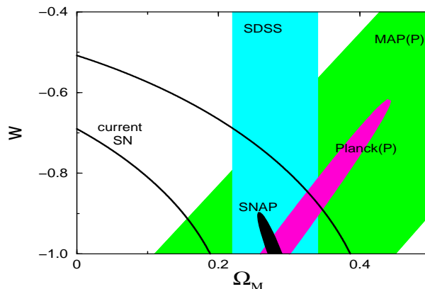
FIG. 1: Projected SNAP constraint compared to those projected for MAP and Planck (with polarization information) and SDSS. Also shown are the present bounds using a total of 54 SNe Ia. All constraints assume a flat Universe with \Omega_M = 1 - \Omega_\phi = 0.28 and constant equation of state factor with fiducial value w = -1 . The plot is taken from Ref. [8], and all contours are 68% confidence intervals.
