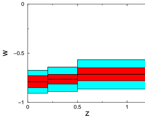
FIG. 3: Here w(z) is parameterized by constant values in redshift bins for the same fiducial model as Fig. 2. The outer region shows 68% cl constraints corresponding to each redshift bin. The inner region shows 68% cl constraints when a Gaussian prior is imposed that penalizes models with a large change in w between two adjacent bins. The plot is taken from Ref. [8].
