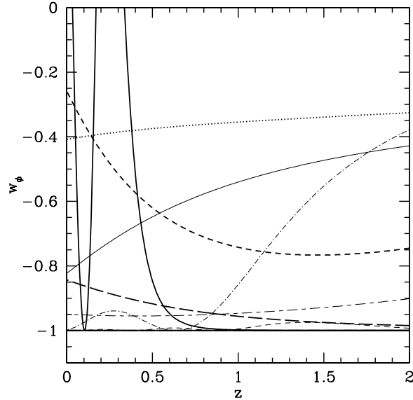
FIG. 4: The redshift evolution of equation of state factor p_\phi = w\rho_\phi for the discussed models. The thin short dash line is the Albrecht & Skordis model [10], the thin dot - short dash line is from the brane inspired potential [10], the thin short dash - long dash line from the potential which involves two exponentials [10], the thick short dashed line from the periodic potential [2], the thick long dashed line from the pure exponential [9], the thick solid line from the Pseudo Nambu-Goldstone Boson potential [2], the thin solid line from the Supergravity inspired potential [4], the thin long dashed line from the exponential tracker solution (underneath w = -1 ) [4], and the thick dotted line from the inverse tracker. The plot is taken from [7].
