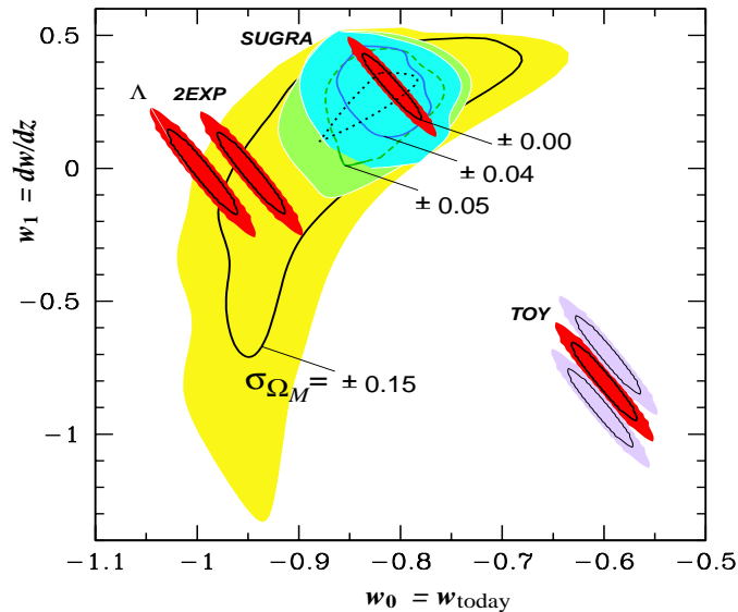
FIG. 7: Separation of dark energy models (labeled as in Fig. 5) in the w_0 - w_1 plane. The contours and shaded regions represent the same probabilities as in Fig. 6. For the Supergravity ( SUGRA ) model, a range of increasingly larger contours represents the results using prior knowledge on \Omega_m with increasingly poorer uncertainty, \sigma_{\Omega_m} . The black dotted curve corresponds to the projected- 1\sigma error contour obtained for more optimistic dataset specifications ( \sigma_{\text{mag}} = 0.09 ; see text) with a prior of 0.25 \leq \Omega_m \leq 0.35 . For the example of the TOY model, flanking contours show the effects of a drifting systematic error (see text). The plot is taken from [6].
